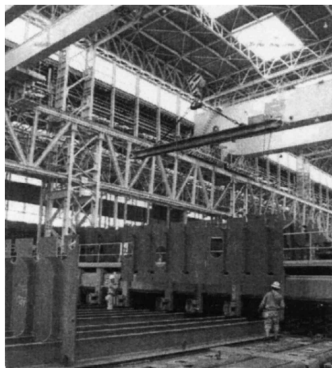
Fig. 3.66. Unit panel and slot construction—sliding on transverses [4]
