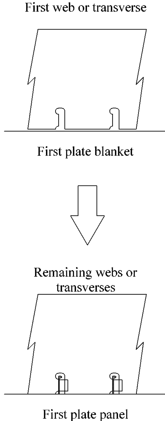
Fig. 3.20. Principal block assembly method 3-1 [2], [30]
