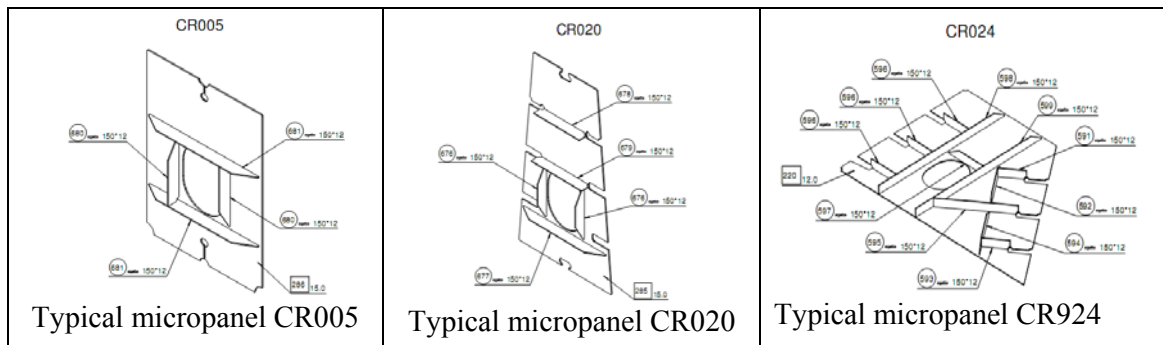
Fig. 4.11 Typical micropanels [30]
