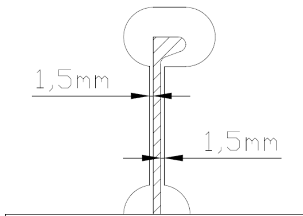
Fig. 3.68. Detail of slot for a bulb profile [10], [30]
