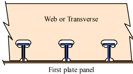
Fig. 3.3. Principal block assembly method 2 [2]
