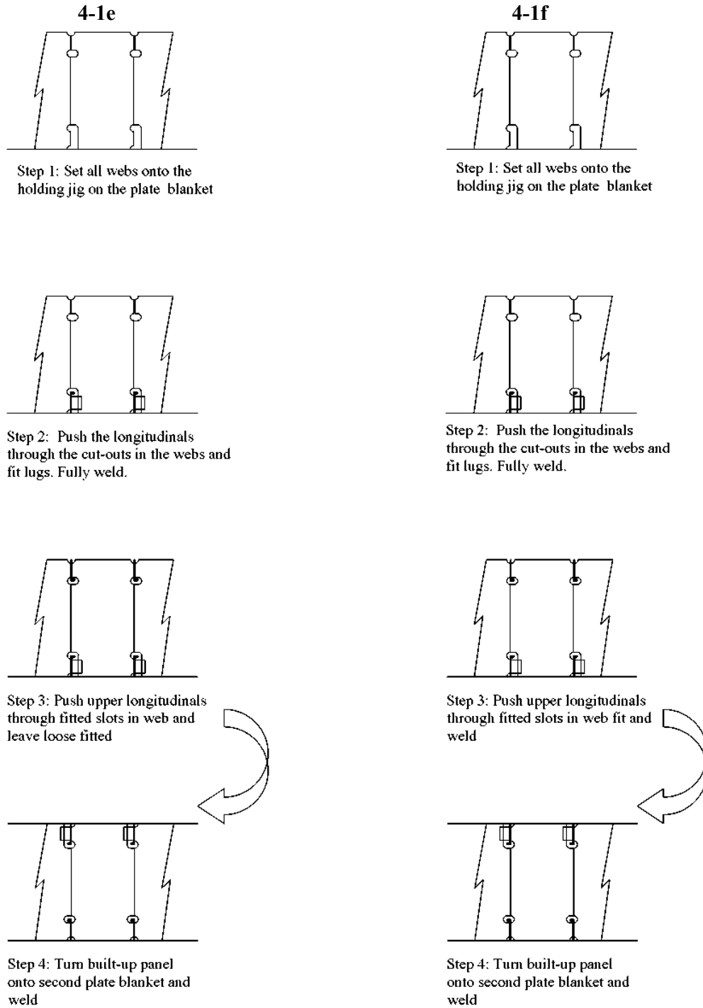
Fig. 3.33. Block assembly methods 4-1e and 4-1f [2], [30]
