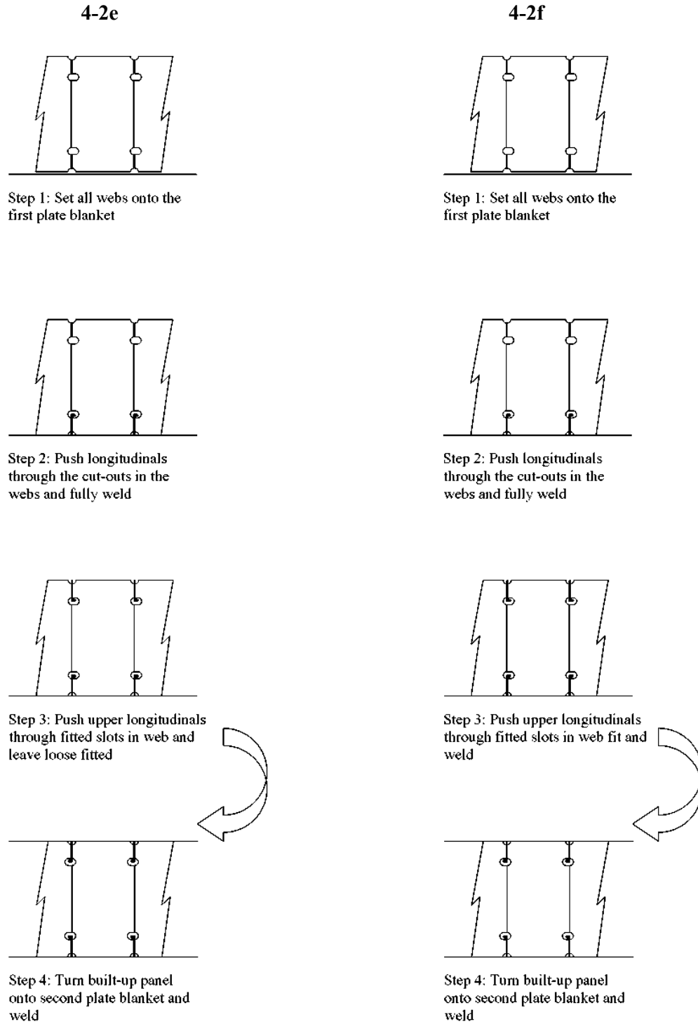
Fig. 3.38. Block assembly methods 4-2e and 4-2f [2], [30]
