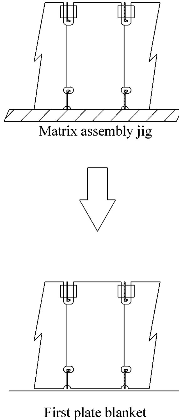
Fig. 3.45. Principal block assembly method 5-2 [2], [30]
