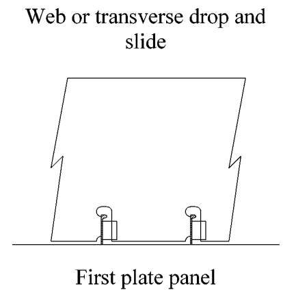
Fig. 3.10. Principal block assembly method 1 [2], [30]
