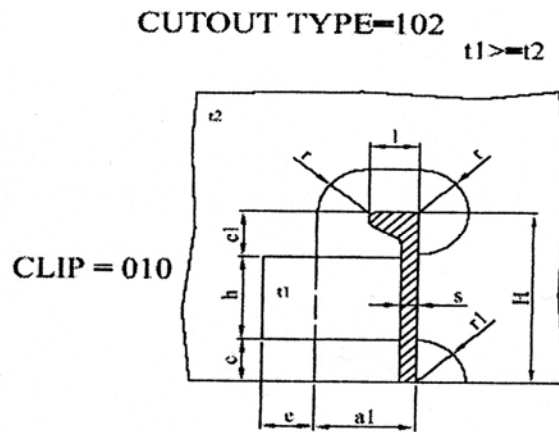
Fig. 7.3. Typical cutout type penetration [30]
