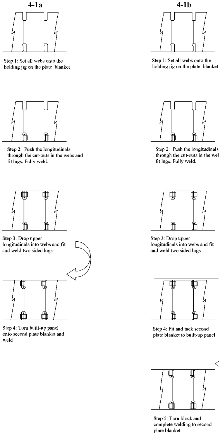
Fig. 3.31. Block assembly method 4-1a and 4-1b [2], [30]
