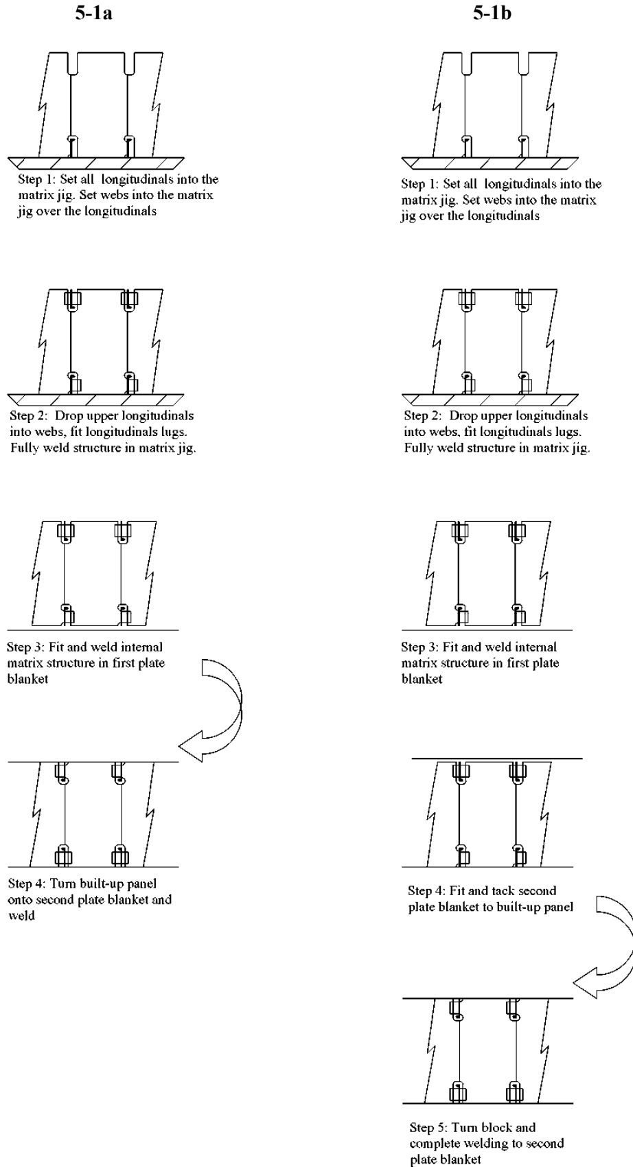
Fig. 3.41. Block assembly methods 5-1a and 5-2b [2], [30]
