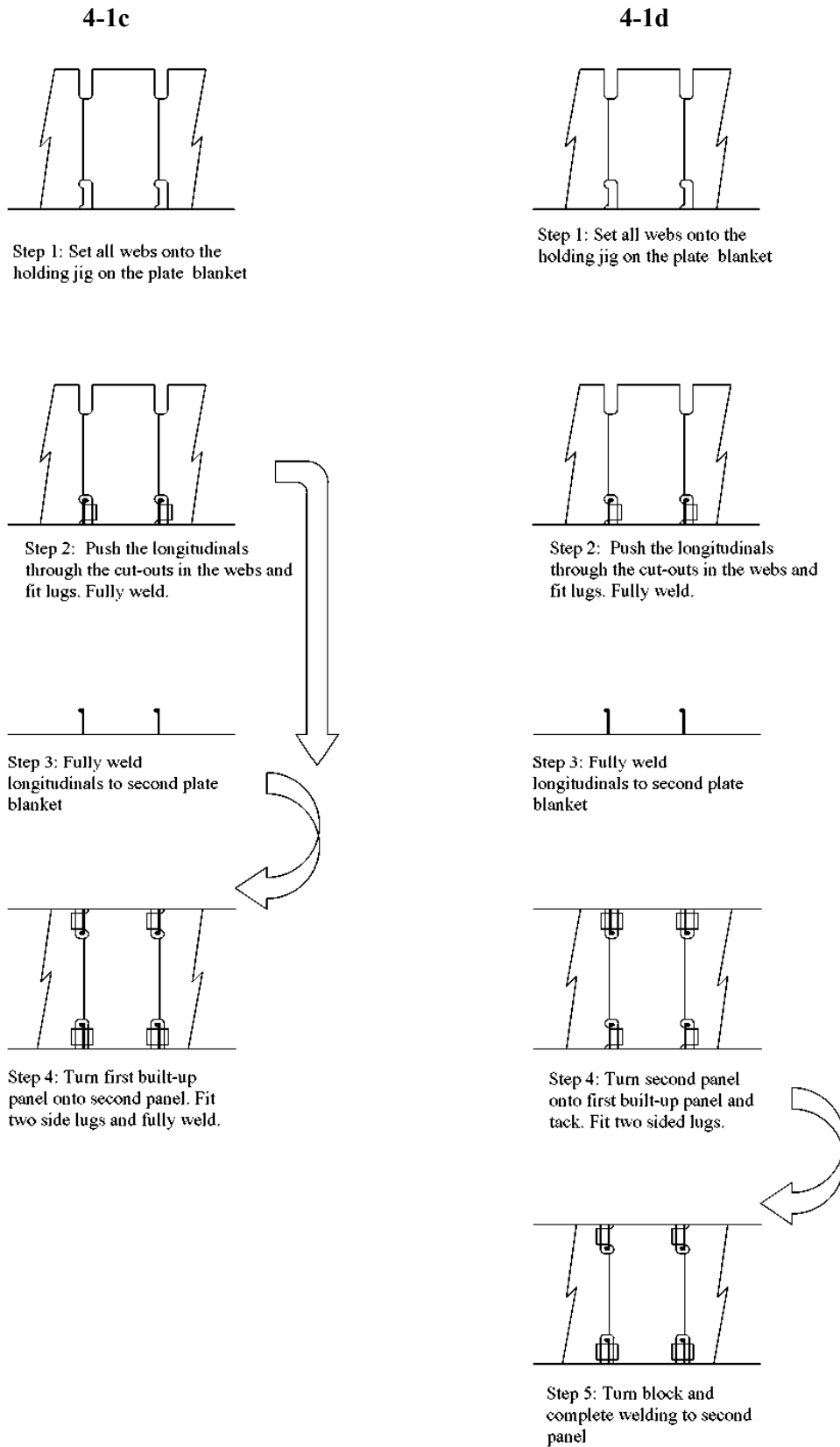
Fig. 3.32. Block assembly methods 4-1c and 4-1d [2], [30]
