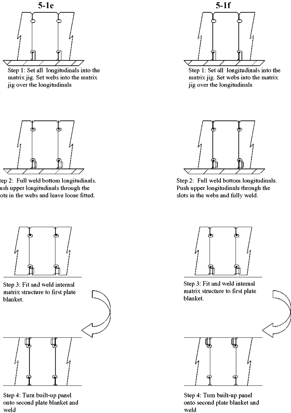
Fig. 3.43. Block assembly methods 5-1e and 5-1f [2], [30]
