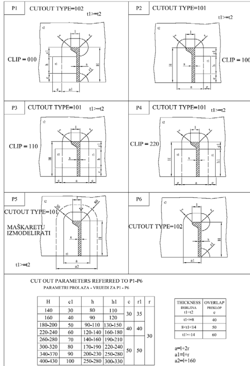
Fig. A1. Shipyard penetration standards [30]
