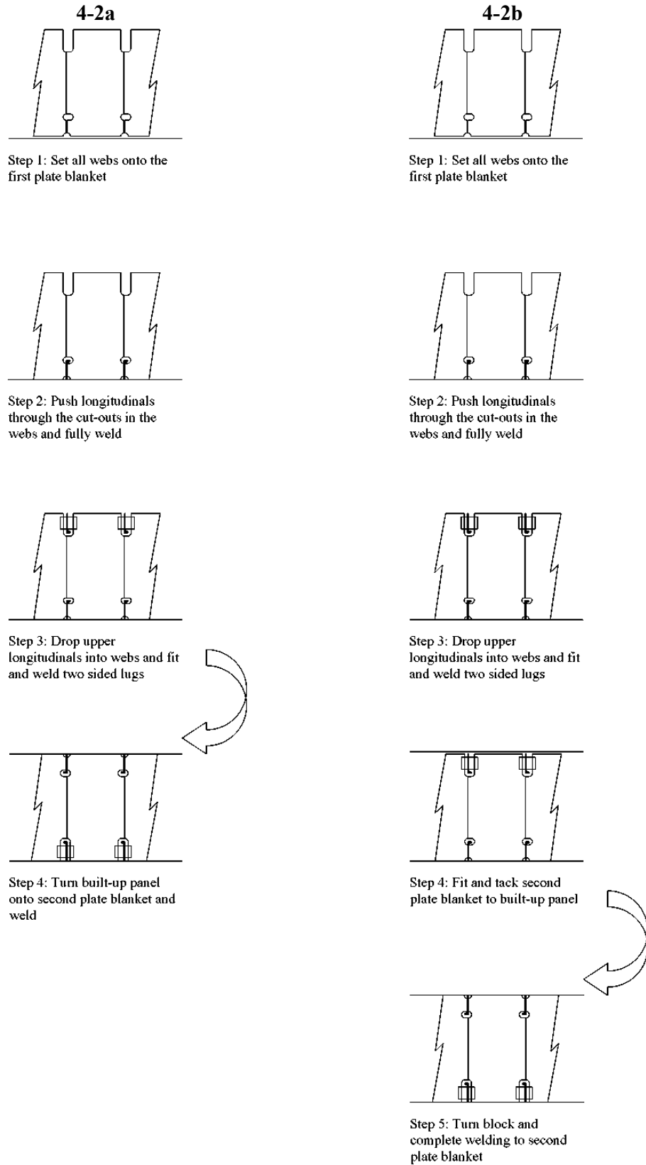
Fig. 3.36. Block assembly methods 4-2a and 4-2b [2], [30]
