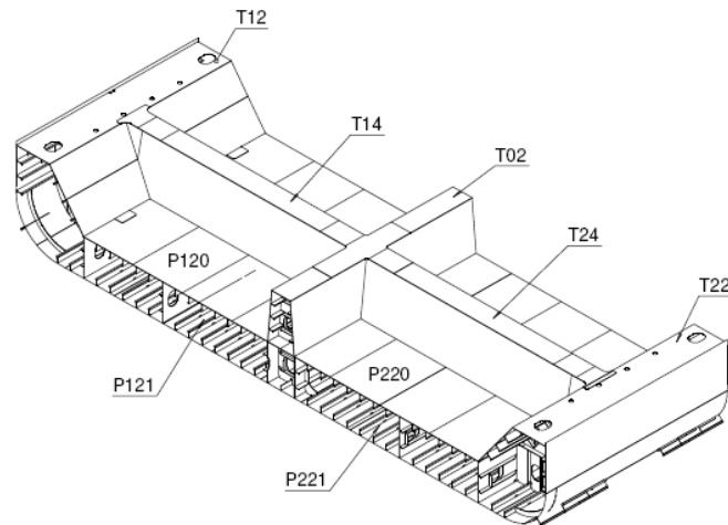
Fig 5.6. The final double bottom block (very large three dimensional section) [30]
