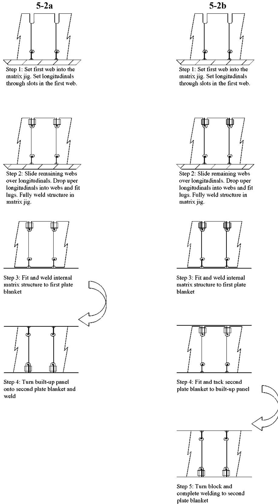
Fig. 3.46. Block assembly methods 5-2a and 5-2b [2], [30]
