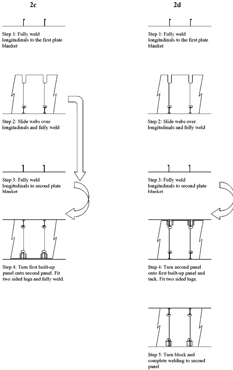
Fig. 3.17. Block assembly methods 2c and 2d [2], [30]
