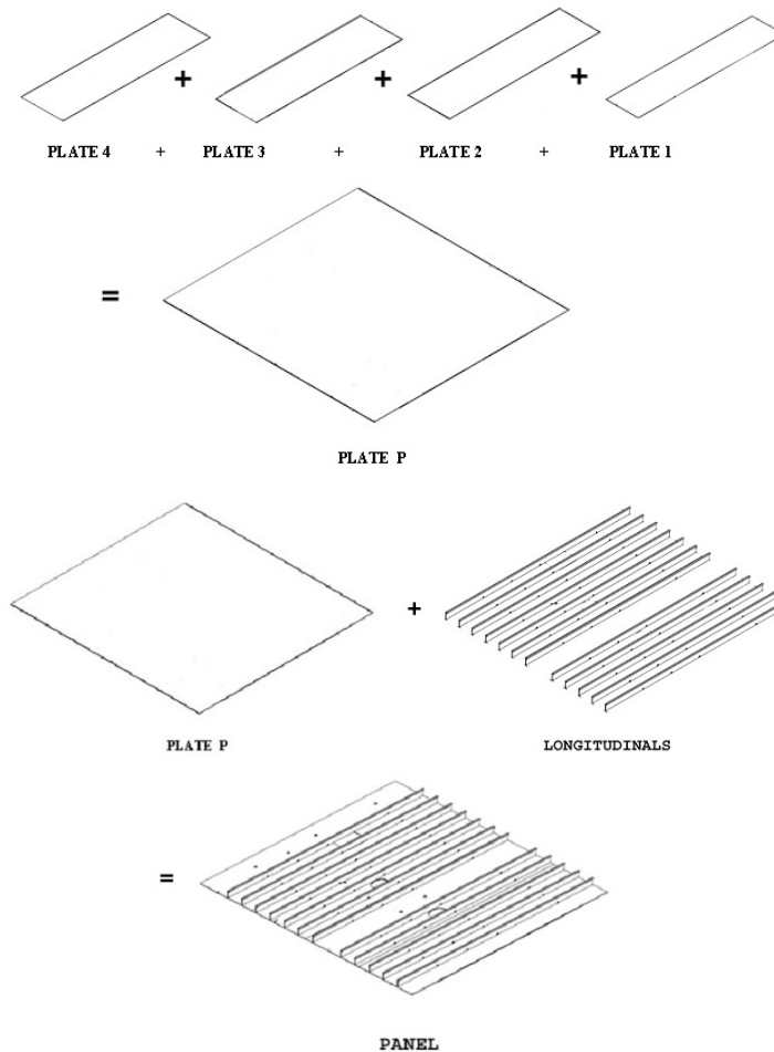
Fig. 5.1. Assembly sequence on the present panel line
