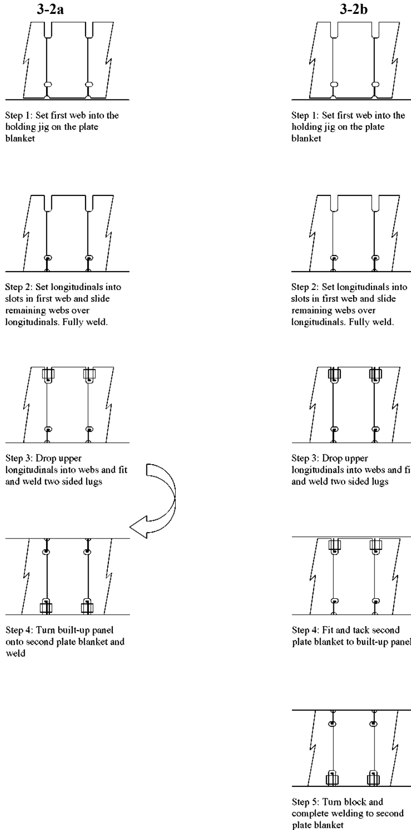
Fig. 3.26. Block assembly methods 3-2a and 3-2b [2], [30]
