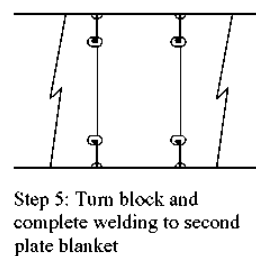
Fig. 3.49. Block assembly method 5-2g [2], [30]
