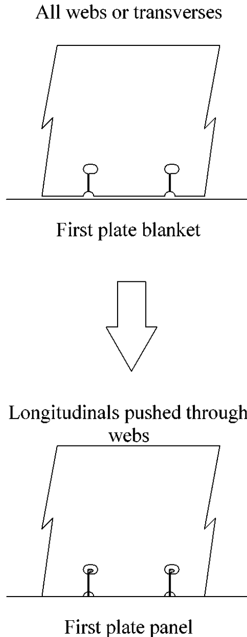
Fig. 3.35. Principal block assembly method 4-2 [2], [30]
