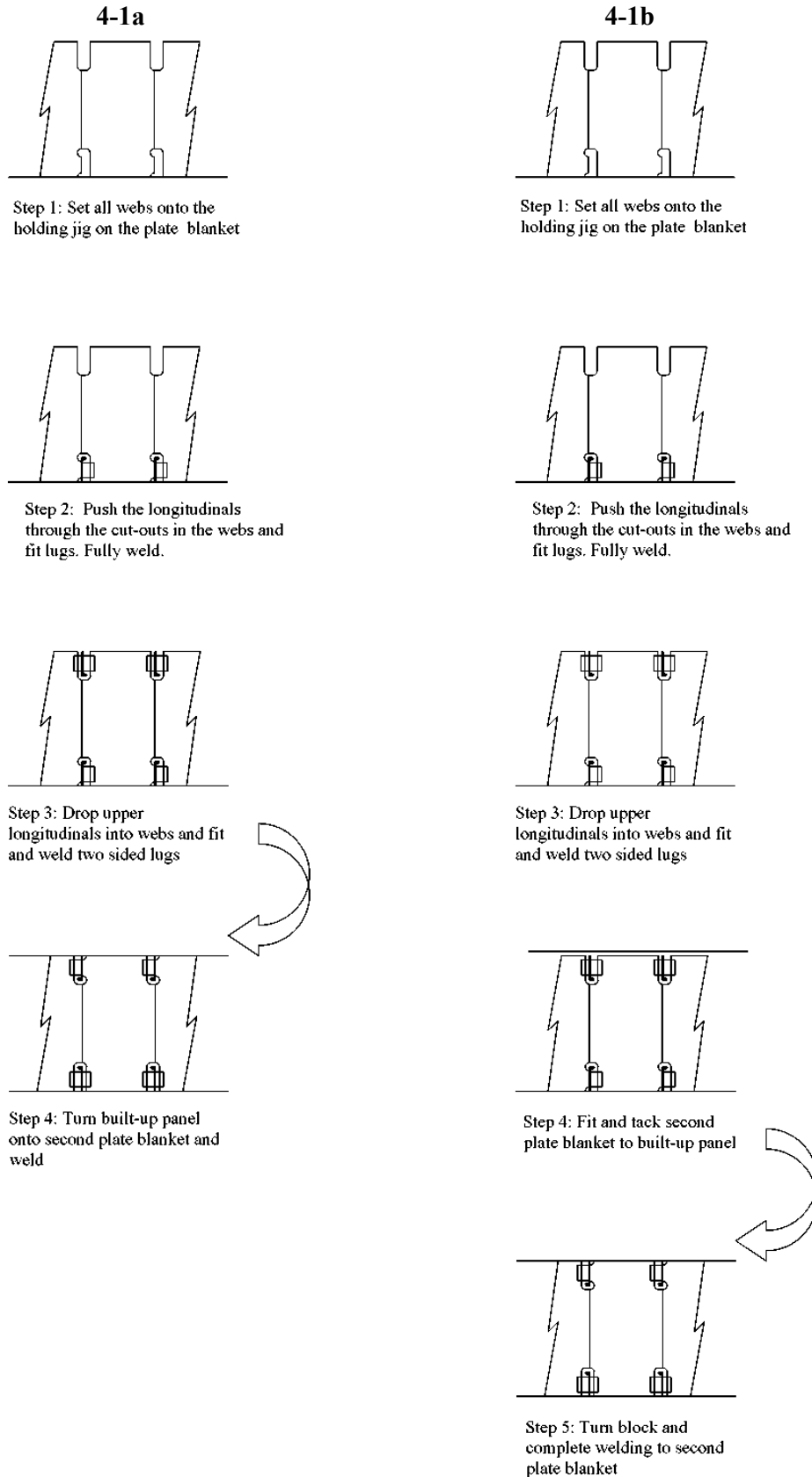
Fig. 3.31. Block assembly method 4-1a and 4-1b [2], [30]
