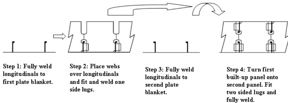
Fig. 7.5. Block assembly method for present state shipyard facilities
