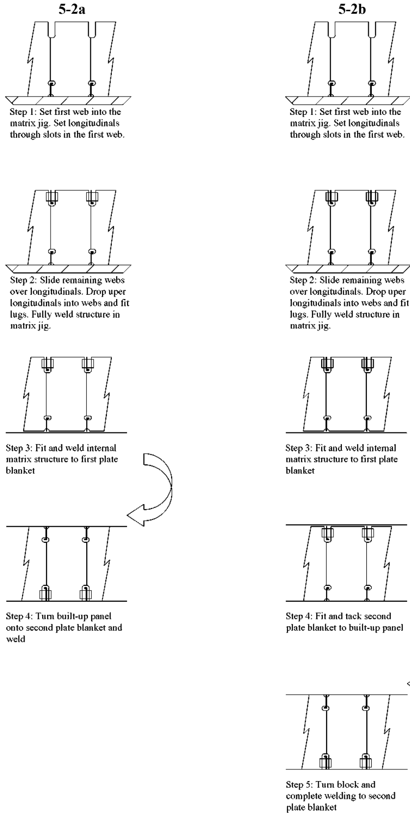
Fig. 3.46. Block assembly methods 5-2a and 5-2b [2], [30]
