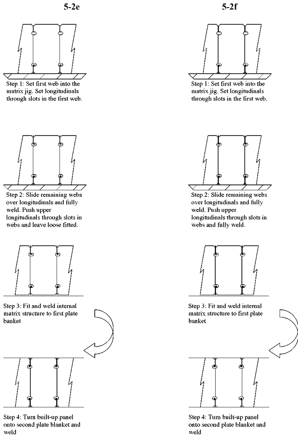
Fig. 3.48. Block assembly methods 5-2e and 5-2f [2], [30]
