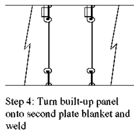
Fig. 3.43. Block assembly methods 5-1e and 5-1f [2], [30]
