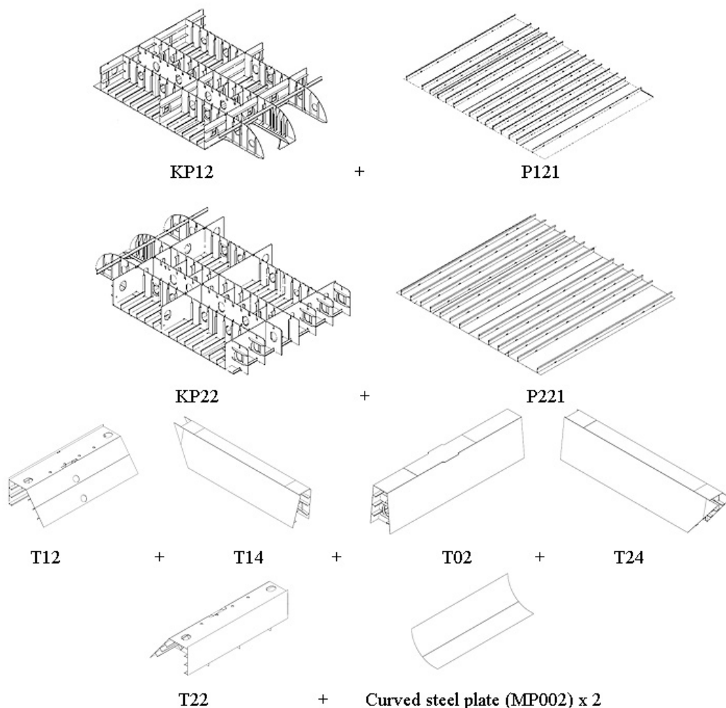
Fig. 5.5. Interim products of the VT double bottom block [30]
